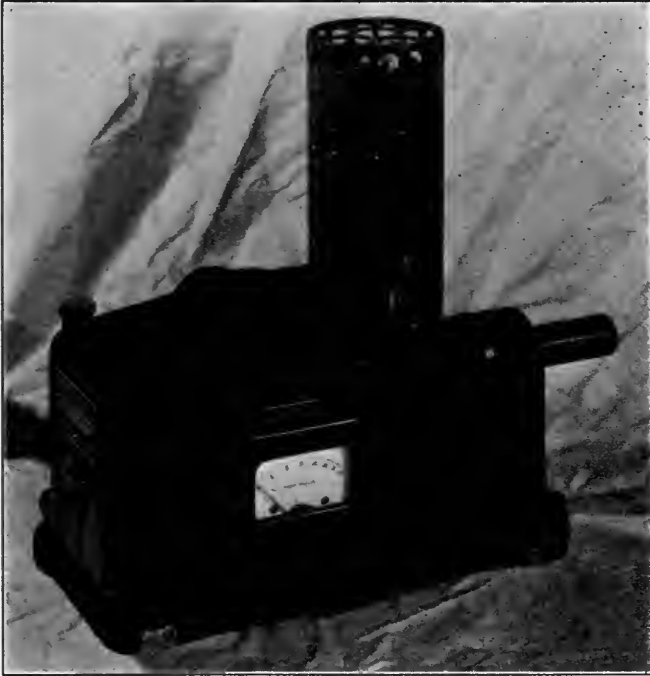
FIG. 10. RCA experimental double-width push-pull variable-area modulator.
